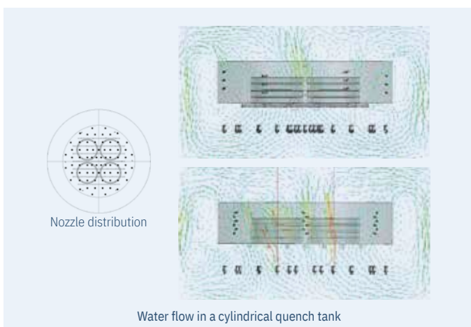
Quench tank
