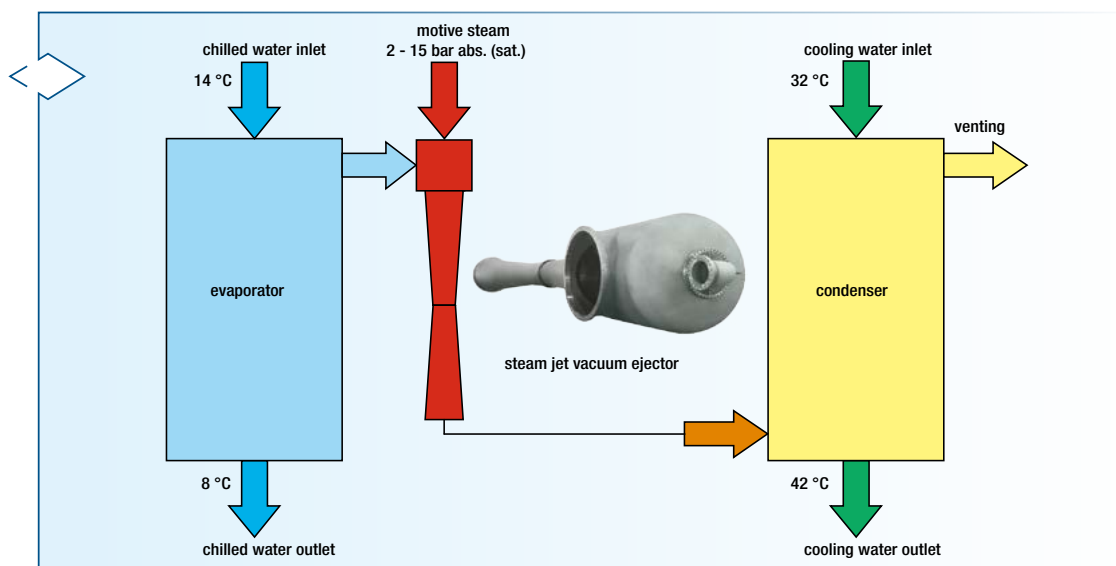
Schematic diagram: steam jet chilling plant
